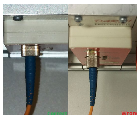
Figure 4a: FC connector correctly lined (green) and not-correctly lined (red)
