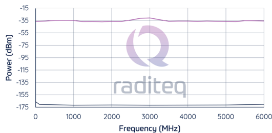
Dynamic range (All Gain stages combined)
