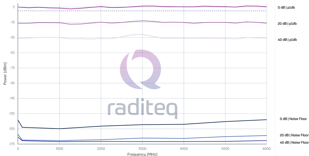
Dynamic range (All Gain stages combined)
